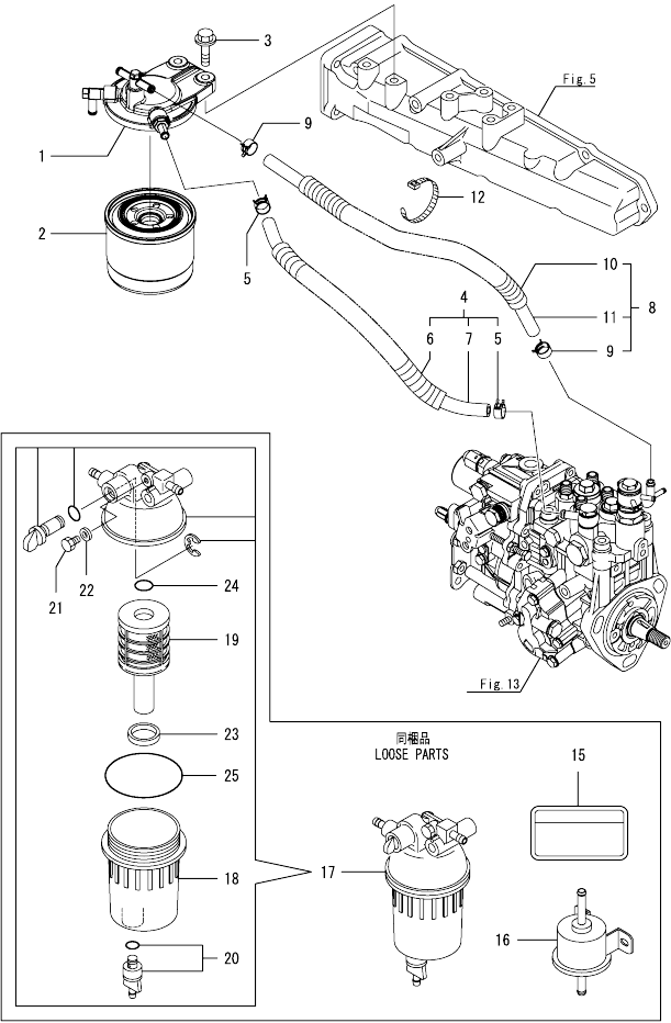
Fig.16. FUEL PIPE
