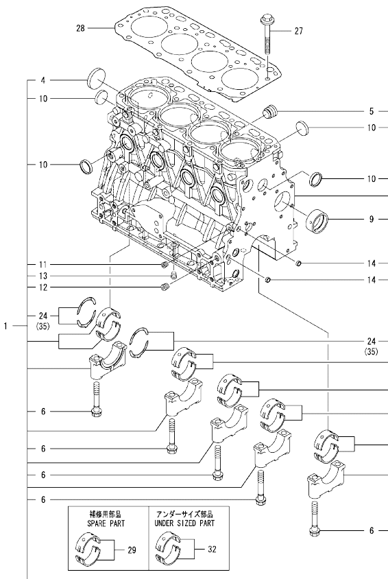
OCD50-M01910 4TNV84T-BGGQ Fig.1. CYLINDER BLOCK
