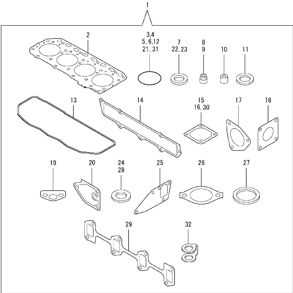
Fig.20. GASKET SET
