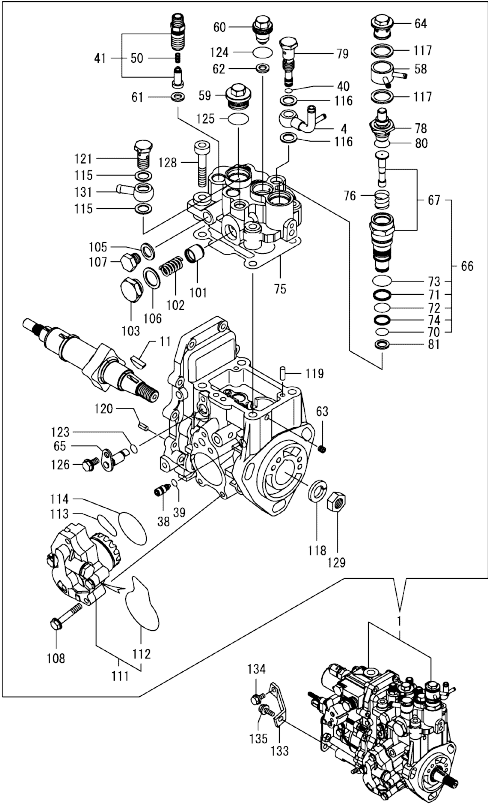
Fig.14. FUEL INJECTION PUMP
