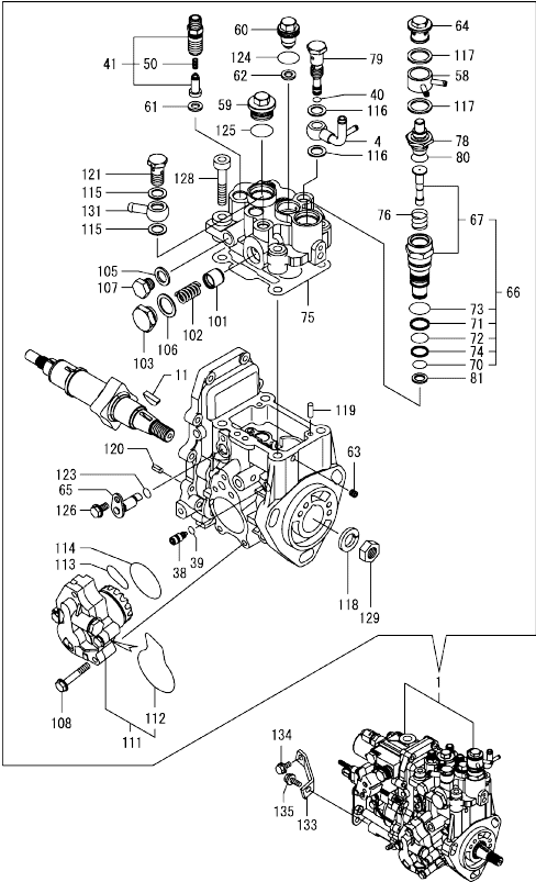
Fig.14. FUEL INJECTION PUMP
