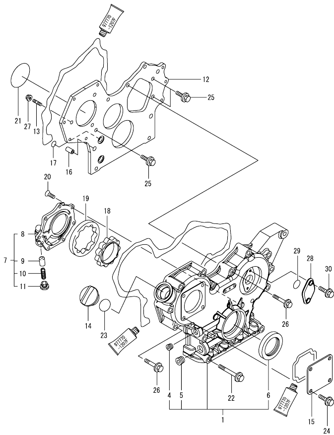
Fig.2. GEAR HOUSING
