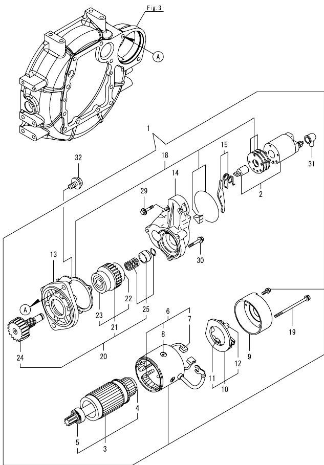
Fig.17. STARTER MOTOR
