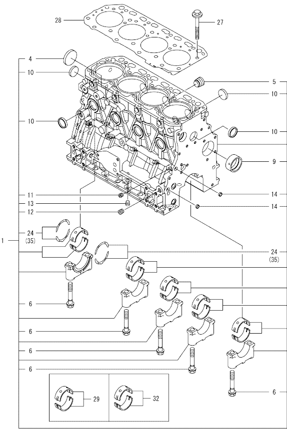
Fig.1. CYLINDER BLOCK
