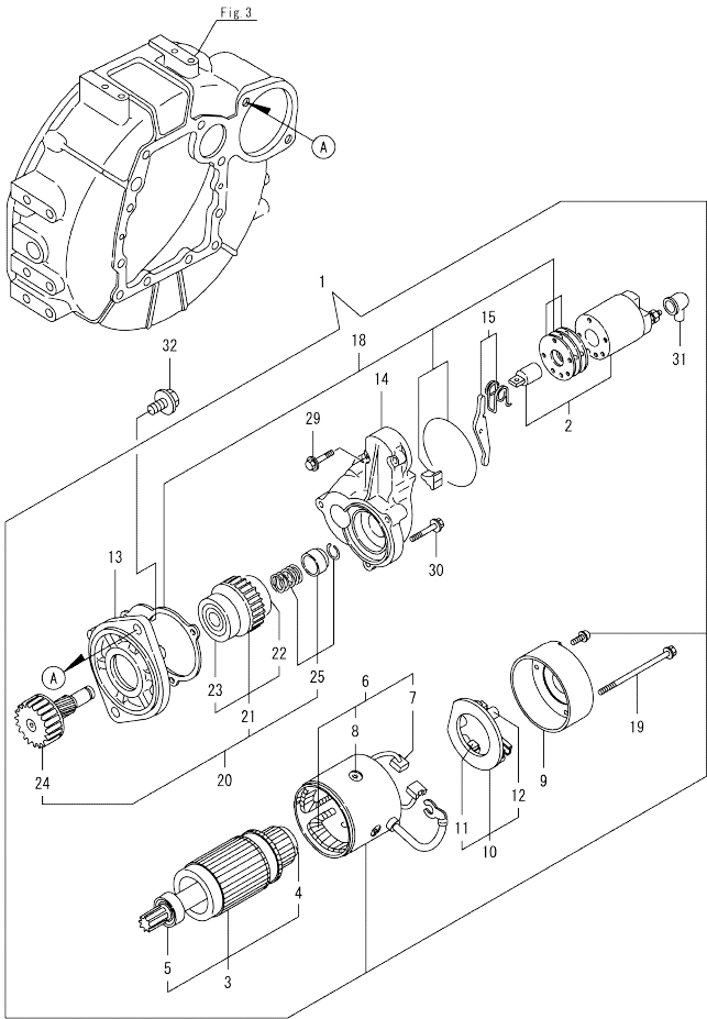
Fig.17. STARTER MOTOR
