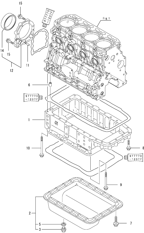
Fig.3. OIL SUMP
