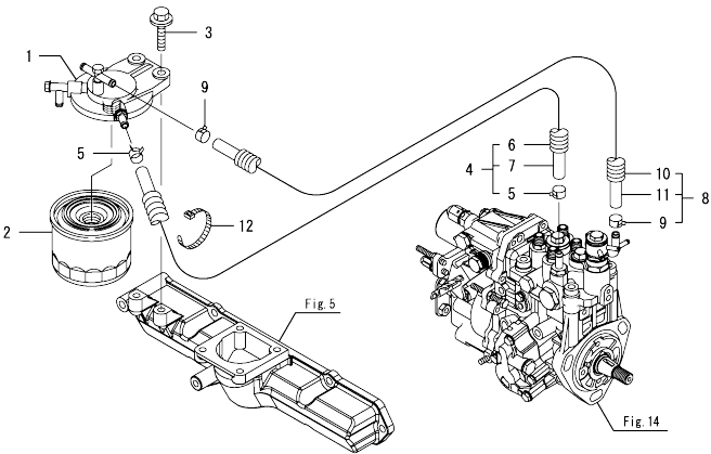
Fig.17. FUEL LINE
