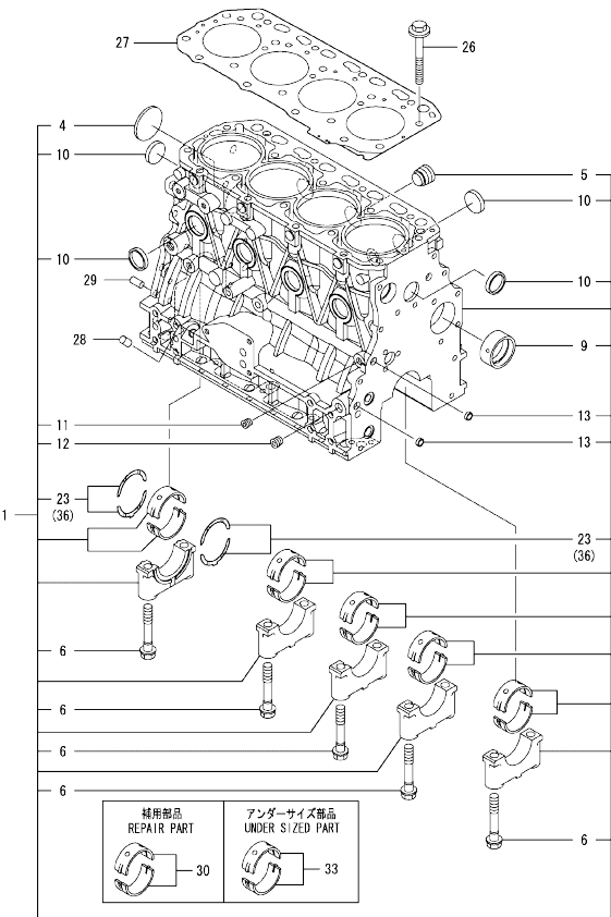
0CW10-M66600 4TNV84T-BMKTF Fig.1. CYLINDER BLOCK
