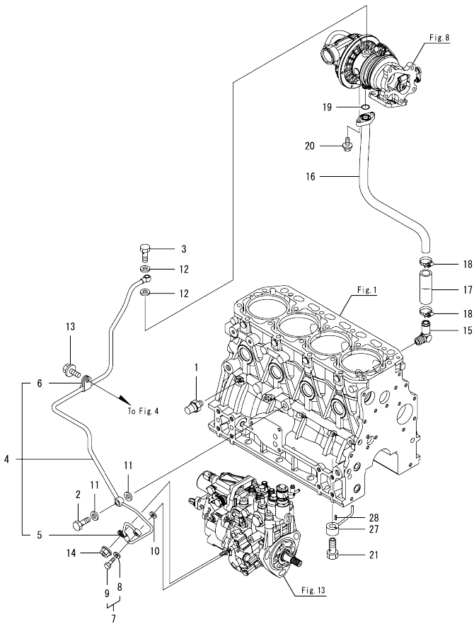
OCD11-M17800 4TNV84T-BPTB Fig.11. LUB.OIL LINE
