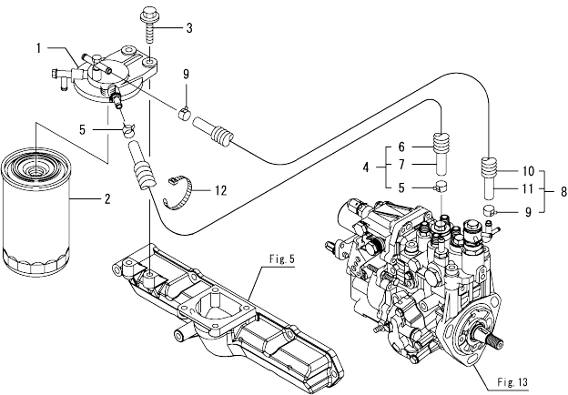
Fig.16. FUEL LINE
