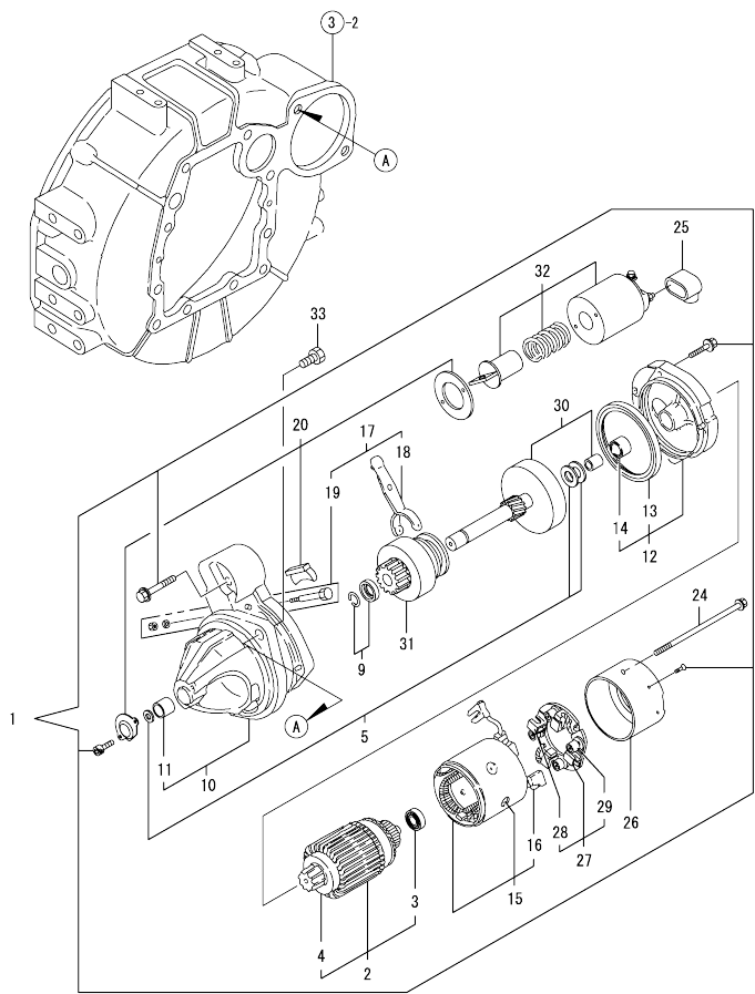
0CW10-M10400 4TNV84T-DFM Fig.17. STARTING MOTOR
