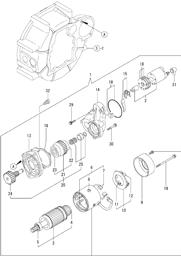
0CW10-M42900 4TNV84T-DSA01 Fig.18. STARTING MOTOR
