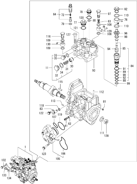
Fig.14. FUEL INJECTION PUMP
