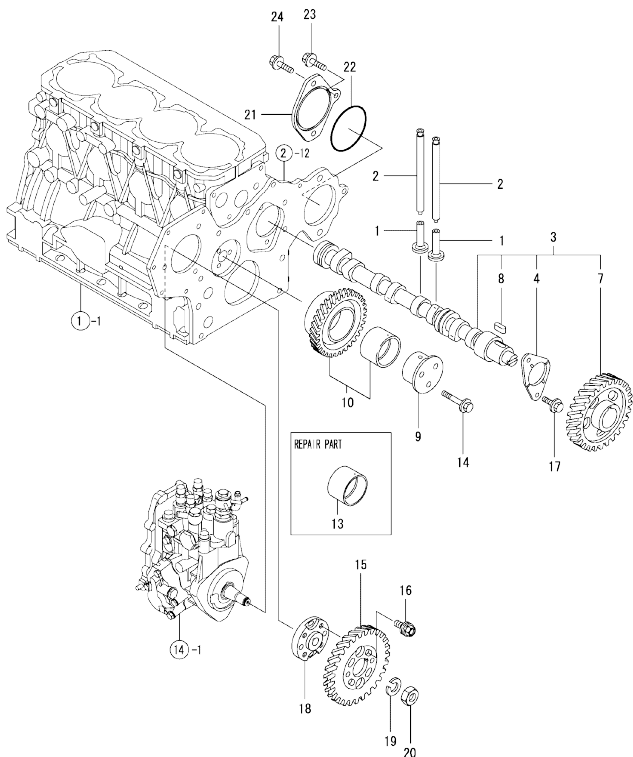
Fig.7. CAMSHAFT & DRIVING GEAR
