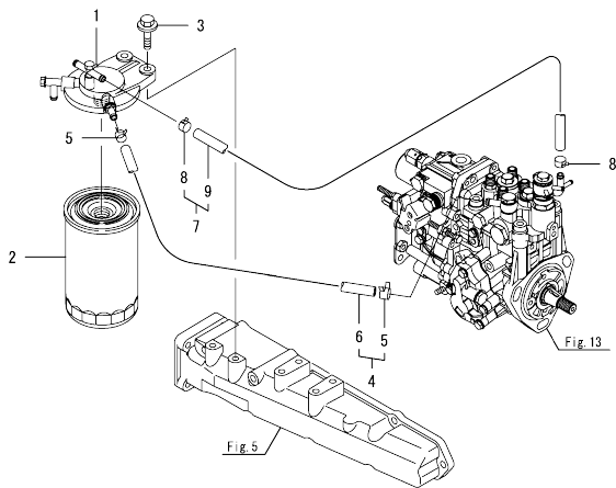
Fig.16. FUEL LINE
