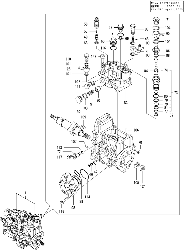
Fig.25. FUEL INJECTION PUMP(INNER PARTS)
