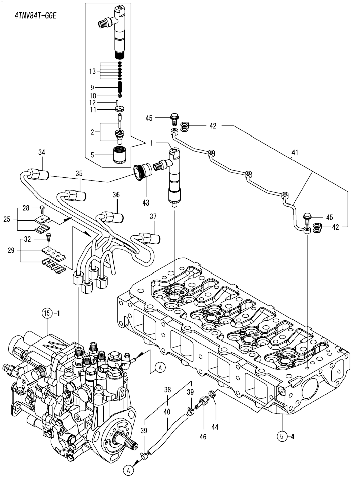
Fig.17. FUEL INJECTION VALVE
