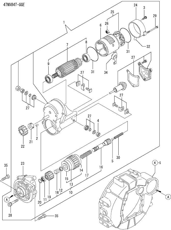
Fig.20. STARTER MOTOR
