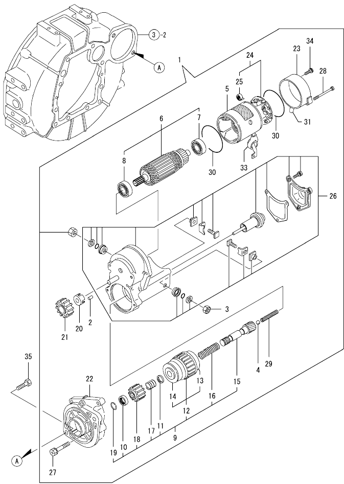
0CW10-M17300 4TNV84T-GGEHC Fig.17. STARTING MOTOR
