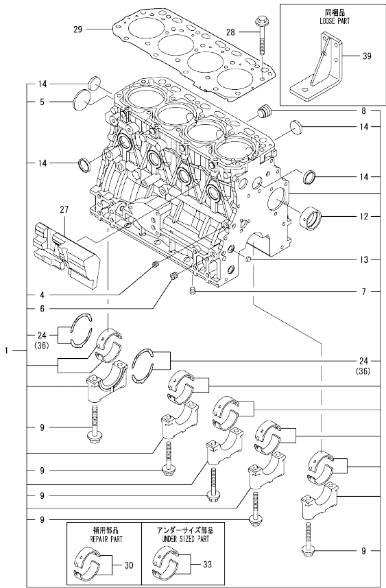
0CW10-M17300 4TNV84T-GGEHC Fig.1. CYLINDER BLOCK
