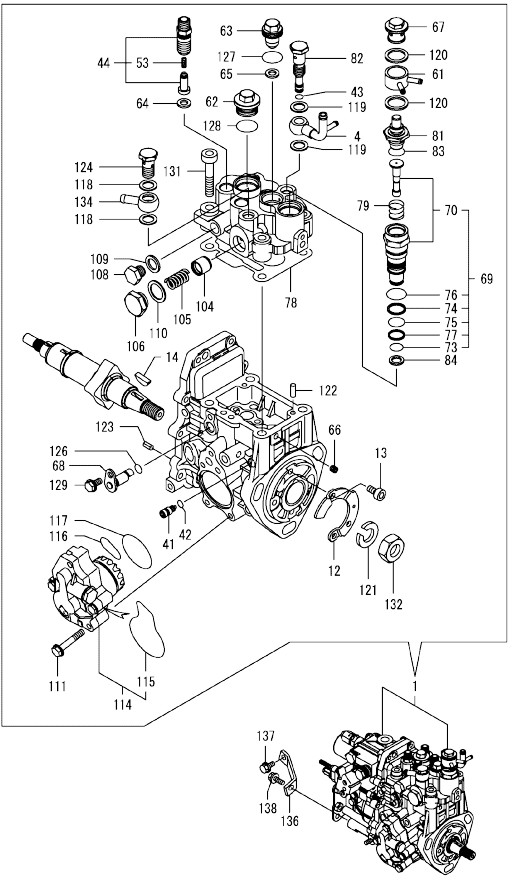
Fig.13. FUEL INJECTION PUMP
