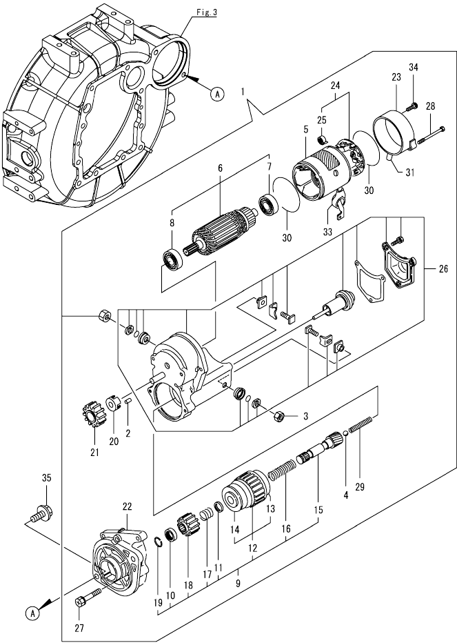
Fig.17. STARTER MOTOR
