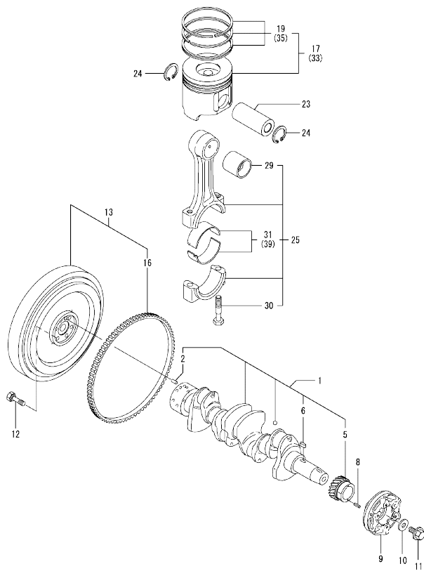
0CW10-M10700 4TNV84T-GKMR Fig.8. CRANKSHAFT & PISTON
