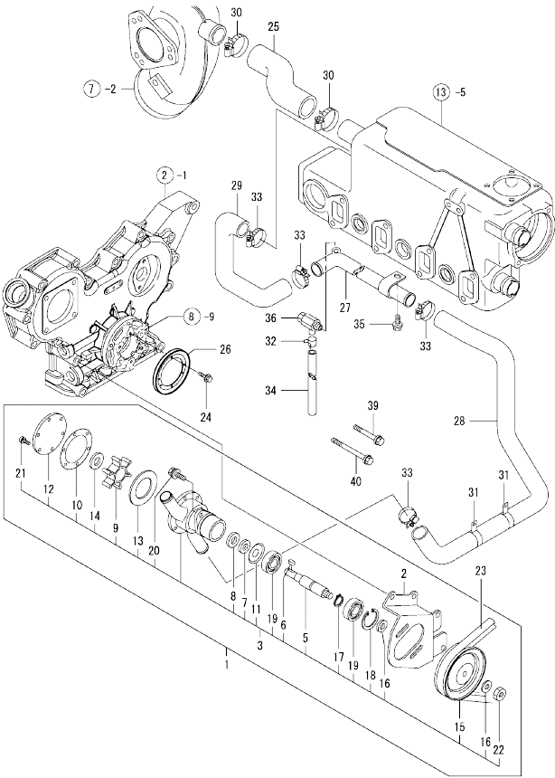
Fig.12. COOLING SEA WATER SYSTEM
