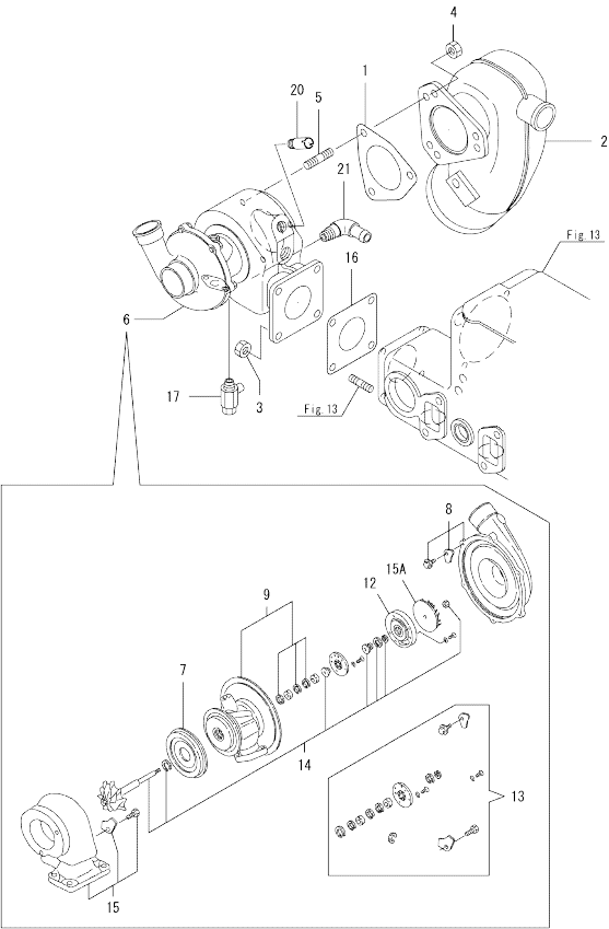
Fig.7. TURBINE
