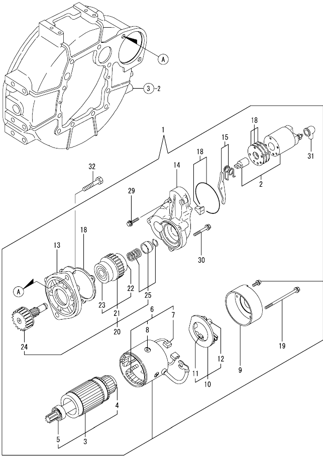
Fig.17. STARTING MOTOR
