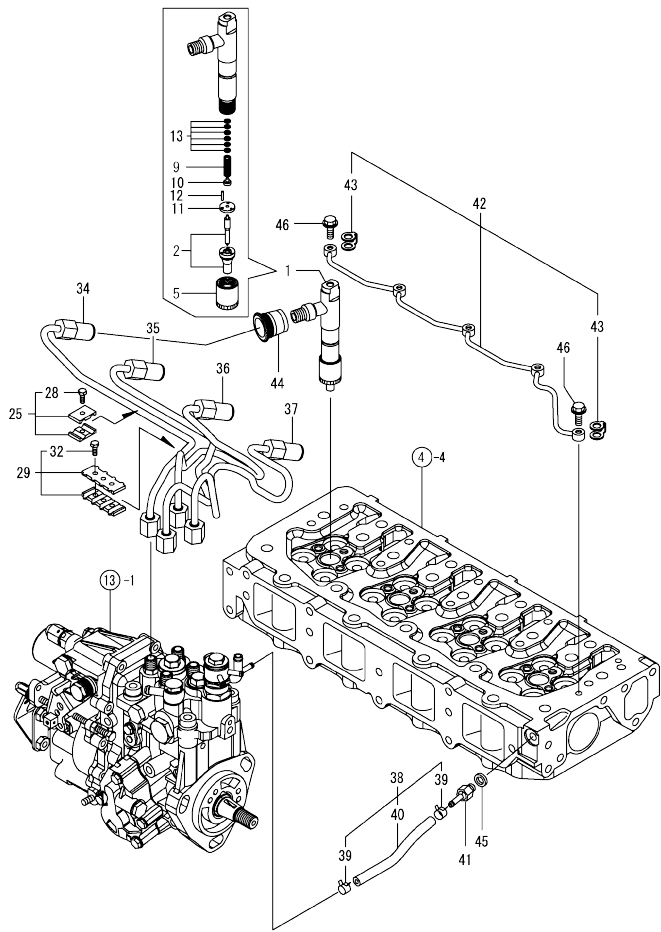
Fig.15. FUEL INJECTION VALVE
