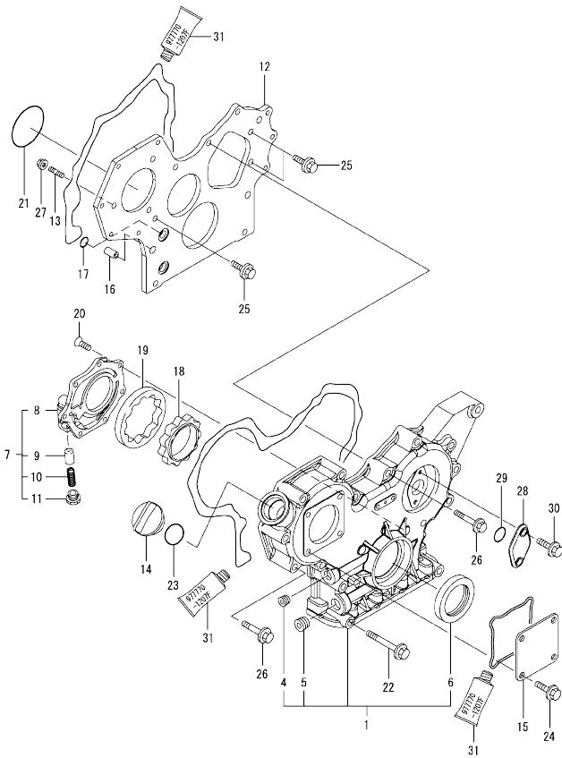
Fig.2. GEAR HOUSING
