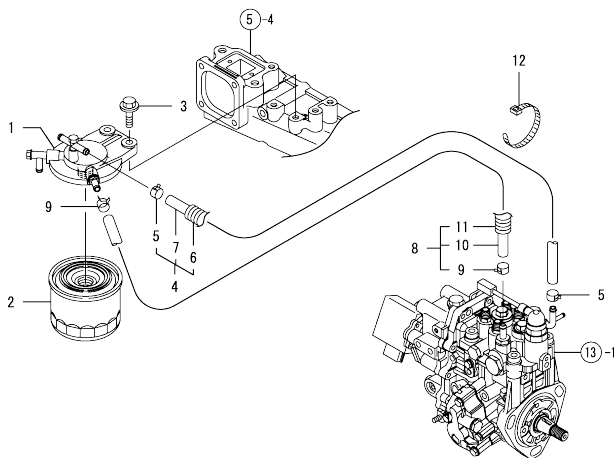
Fig.16. FUEL LINE
