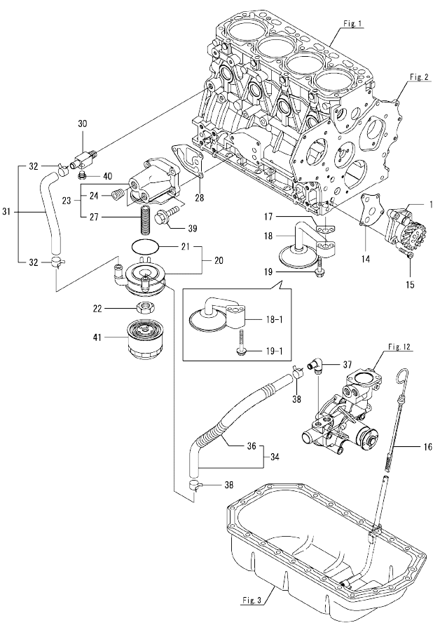
OCD11-M10502 4TNV84T-ZXGYB Fig.10. LUB. OIL SYSTEM
