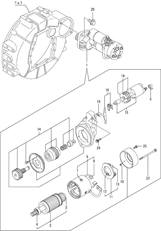
OCD11-M10502 4TNV84T-ZXGYB Fig.17. STARTER MOTOR
