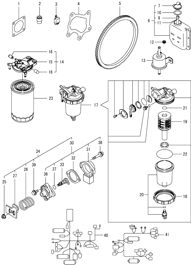
Fig.19. ACCESSORY
