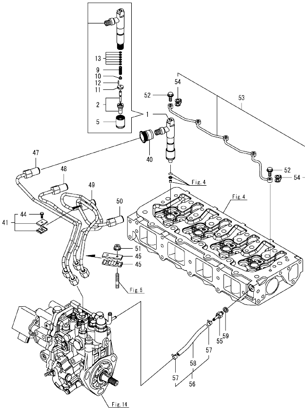
Fig.16. FUEL INJECTION VALVE
