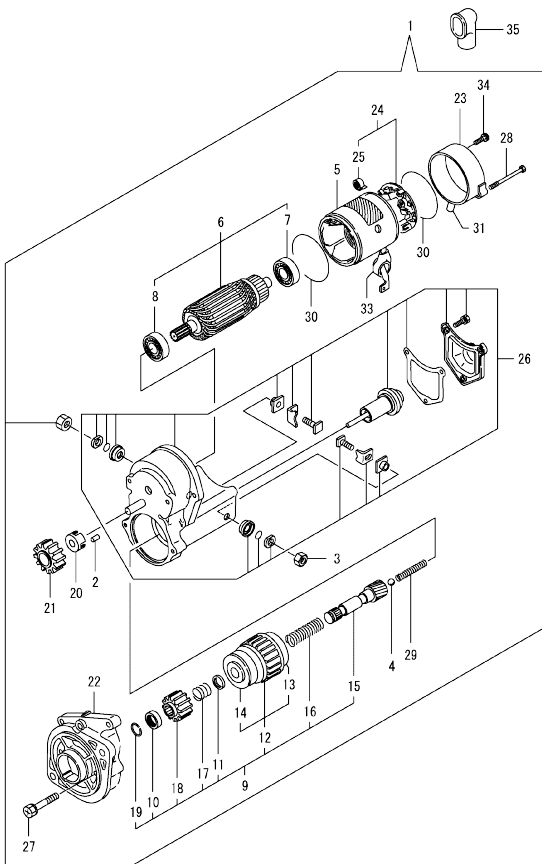
Fig.18. STARTER MOTOR
