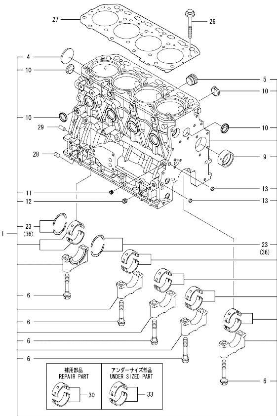
Fig.1. CYLINDER BLOCK
