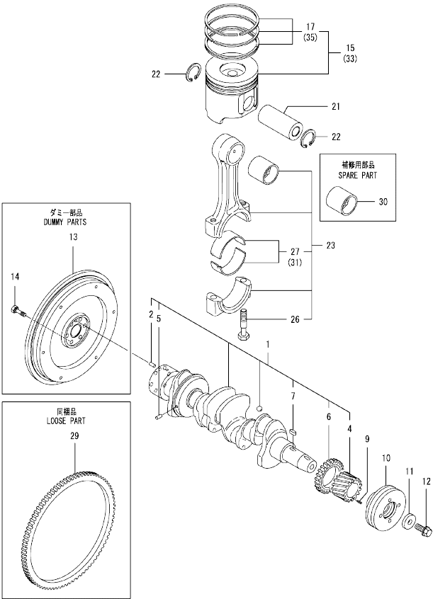
Fig.9. CRANKSHAFT & PISTON
