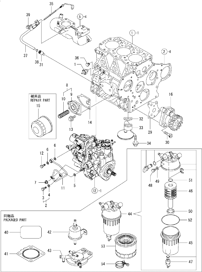
Fig.10. LUB.OIL SYSTEM
