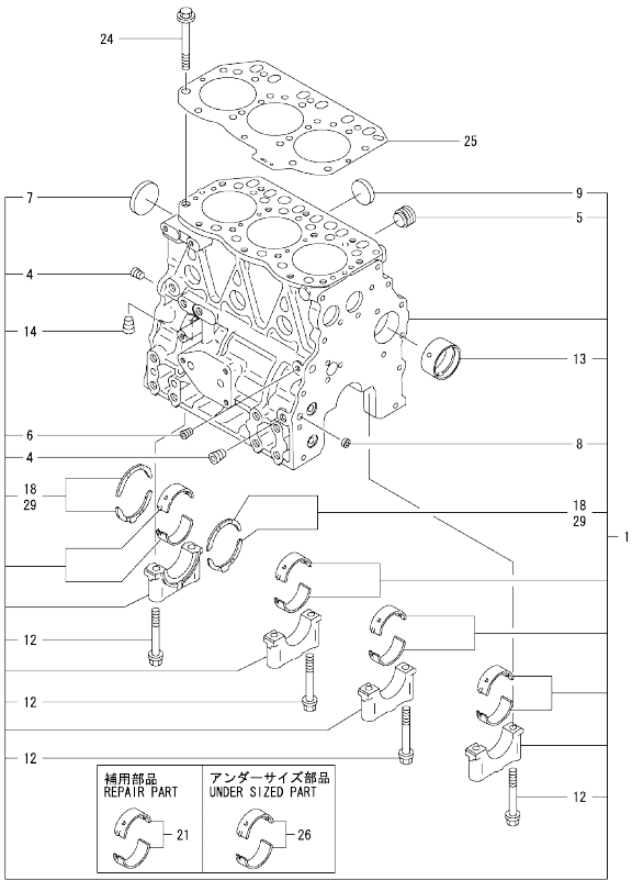
Fig.1. CYLINDER BLOCK
