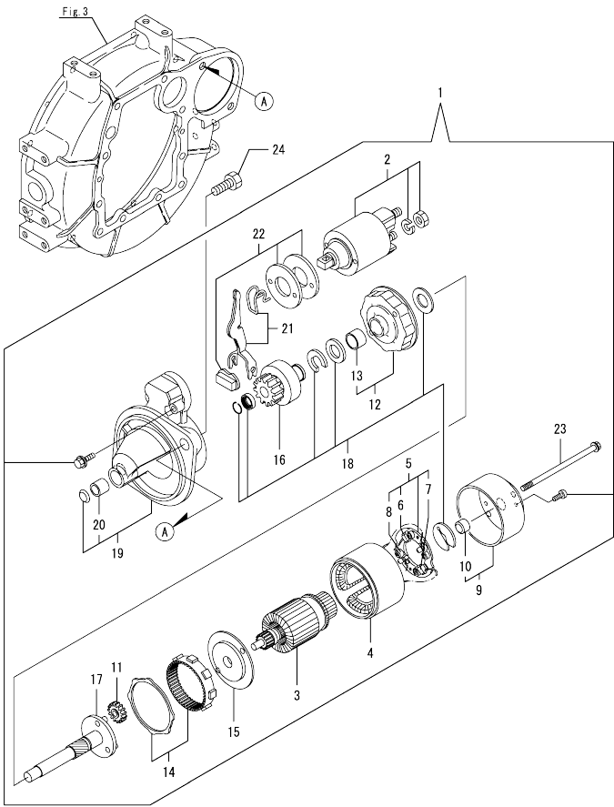
OCD11-M07401 3TNV82A-BPYB Fig.15. STARTER MOTOR
