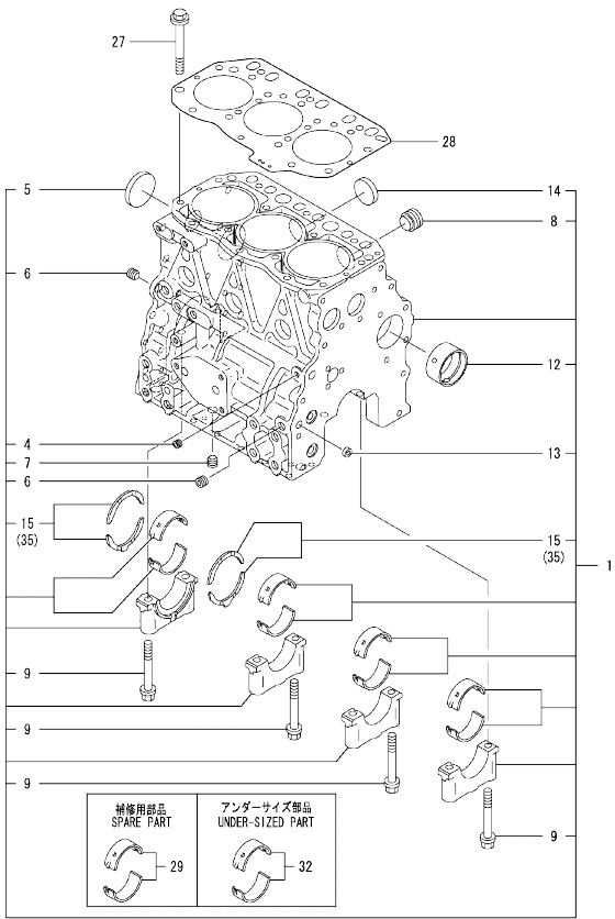
OCD11-M07401 3TNV82A-BPYB Fig.1. CYLINDER BLOCK
