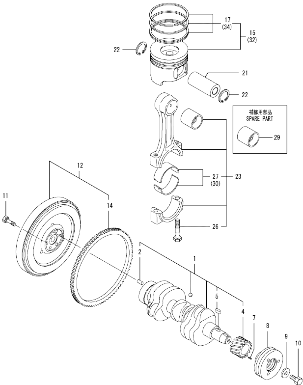
Fig.8. CRANKSHAFT & PISTON
