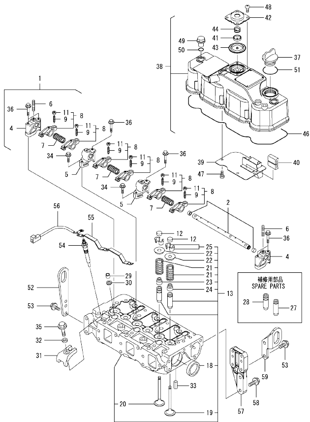
Fig.18. (4A)CYLINDER HEAD & BONNET
