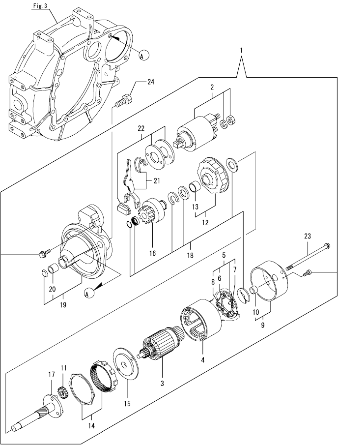
Fig.15. STARTER MOTOR
