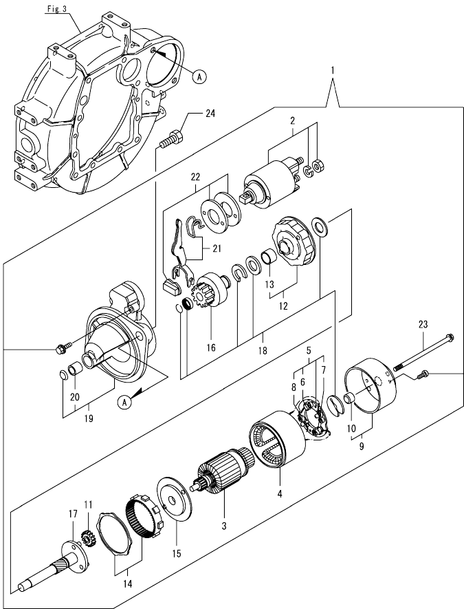
Fig.15. STARTER MOTOR
