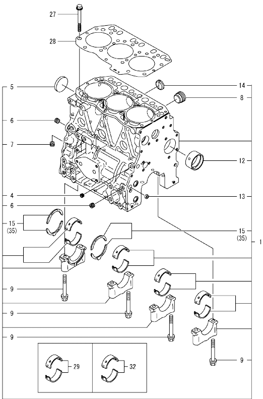
Fig.1. CYLINDER BLOCK
