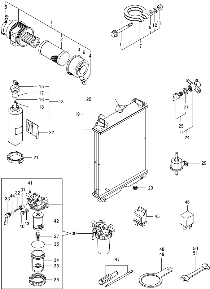
Fig.18. ACCESSORY
