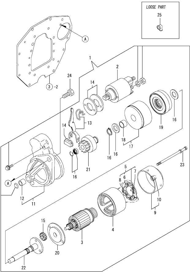
Fig.14. STARTING MOTOR
