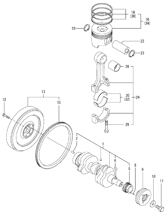
Fig.8. CRANKSHAFT & PISTON
