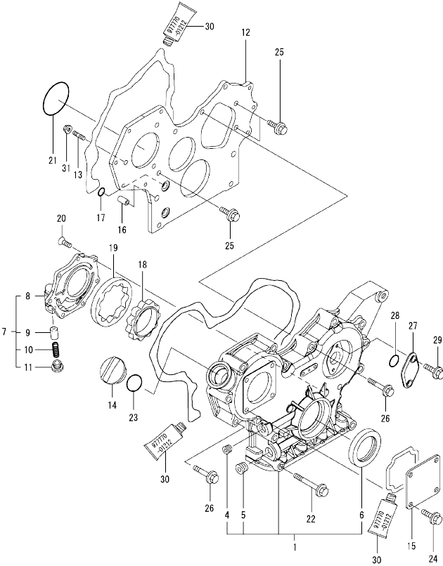
OCR10-M60400 3TNV82A-DMW Fig.2. GEAR HOUSING
