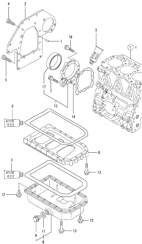
Fig.3. MOUNTING FLANGE & OIL SUMP
