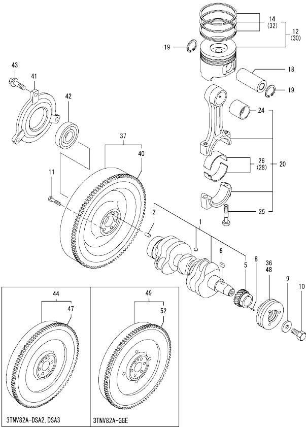
Fig.9. CRANKSHAFT & PISTON
