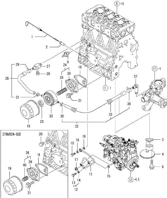
Fig.10. LUB. OIL SYSTEM
