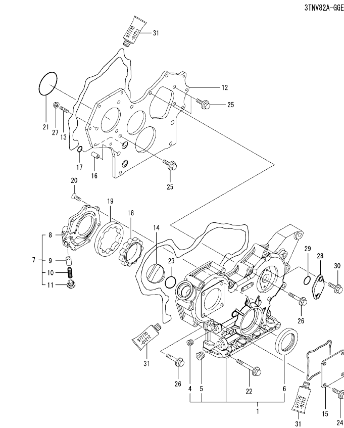
Fig.3. GEAR HOUSING
