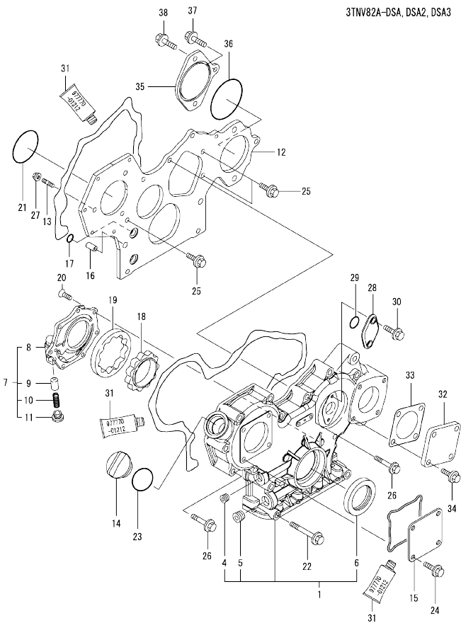
Fig.2. GEAR HOUSING
