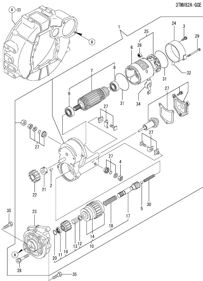
Fig.17. STARTER MOTOR
