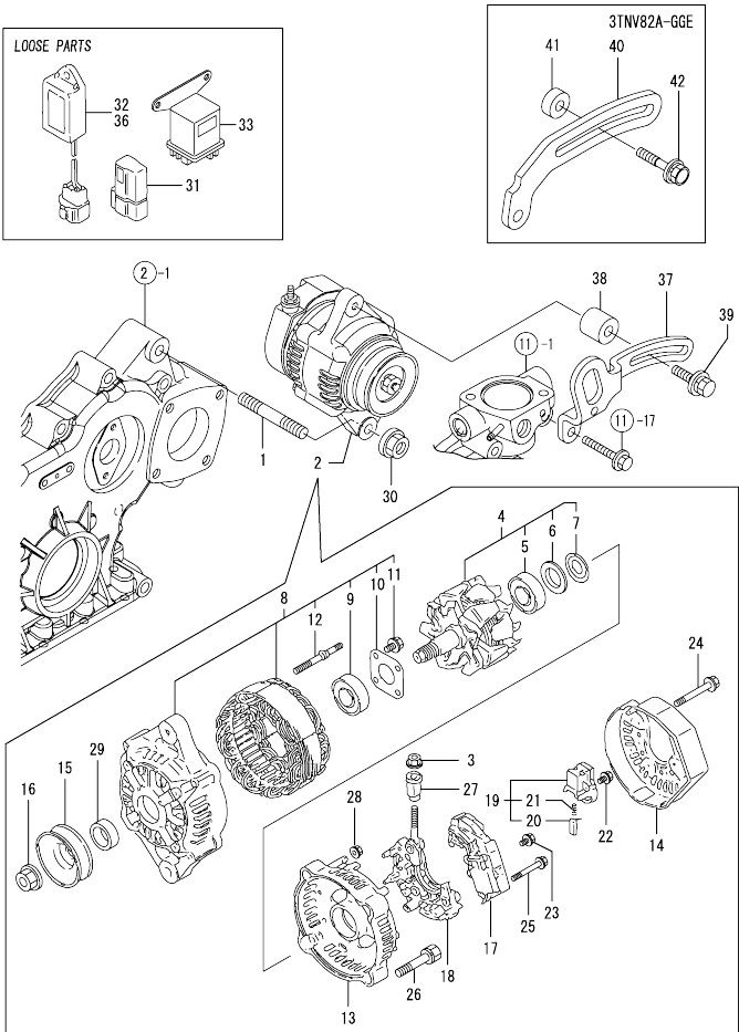
OCR10-M56200 ENGINE Fig.18. GENERATOR
