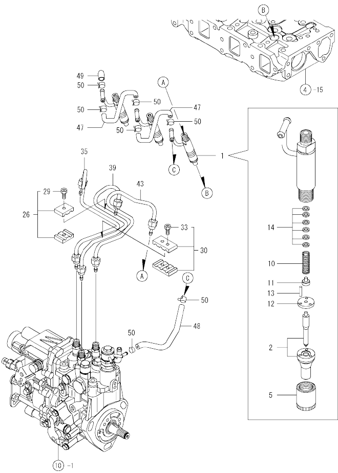
Fig.11. FUEL INJECTION VALVE
