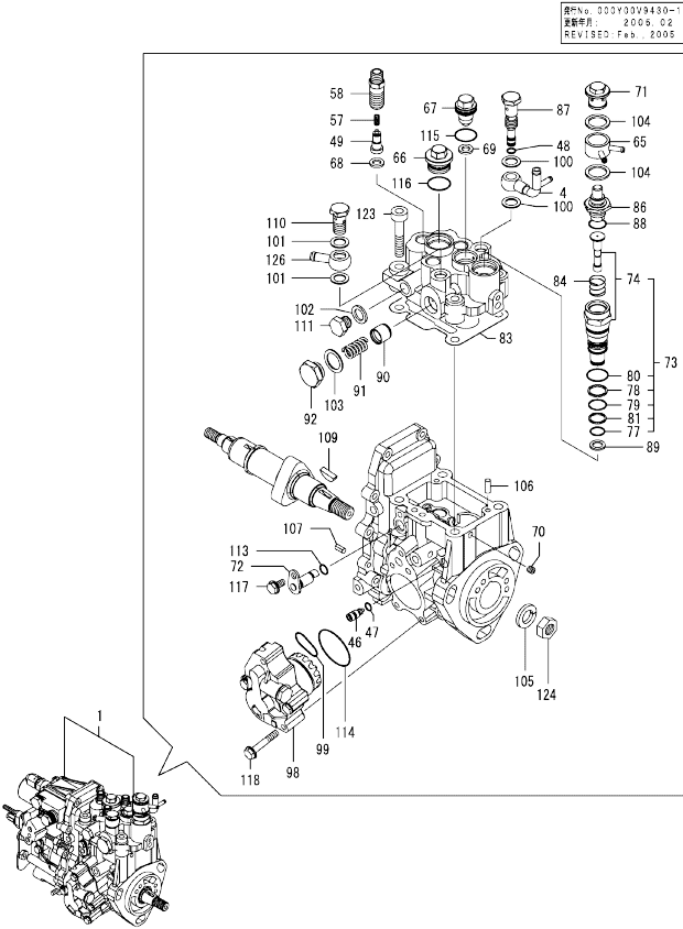
Fig.16. FUEL INJECTION PUMP(INNER PARTS)
