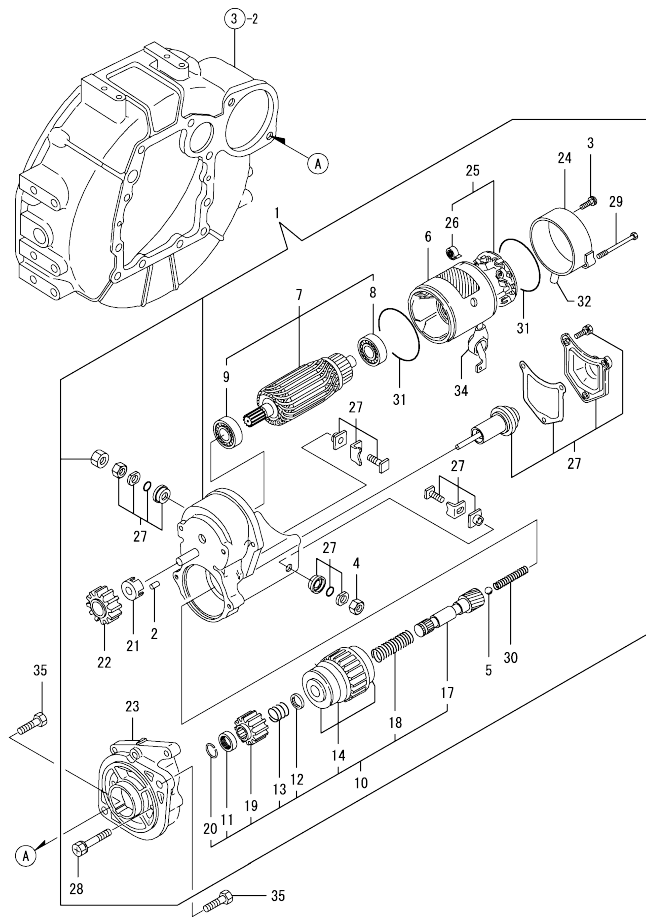
Fig.15. STARTING MOTOR
