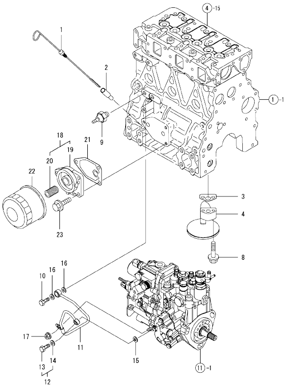
Fig.9. LUB.OIL SYSTEM
