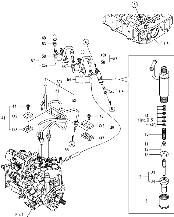
Fig.13. FUEL INJECTION VALVE
