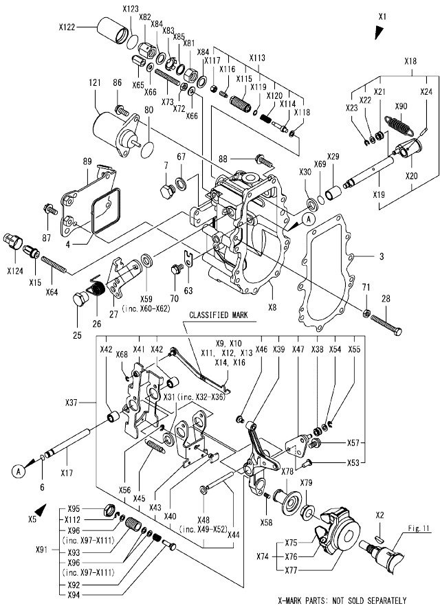
OCD50-M03480 ENGINE Fig.12. GOVERNOR
