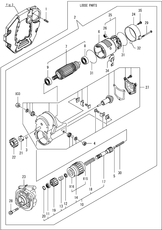
Fig.15. STARTER MOTOR
