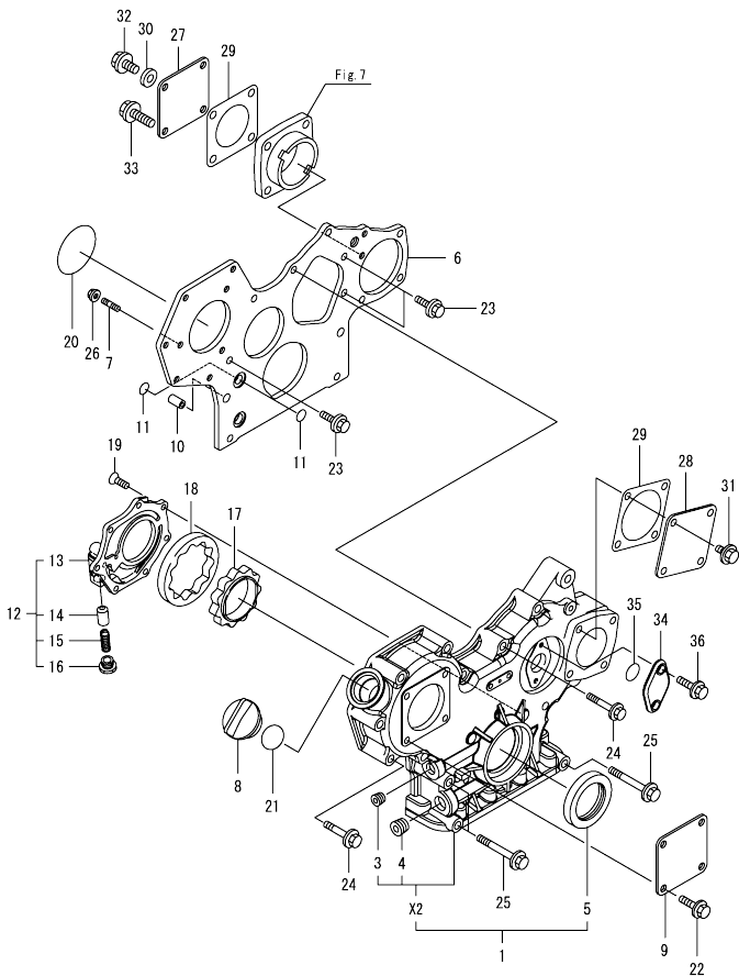
Fig.2. GEAR HOUSING
