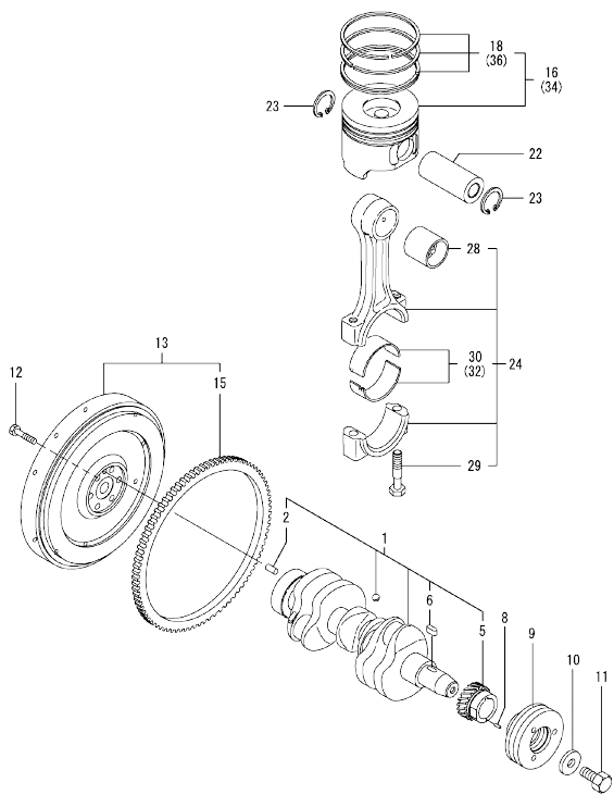
Fig.8. CRANKSHAFT & PISTON
