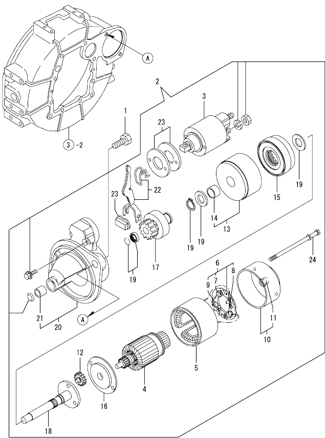
Fig.14. STARTING MOTOR
