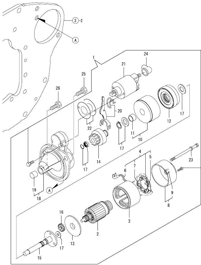
OCR10-M60300 3TNV82A-MU1 Fig.16. STARTING MOTOR
