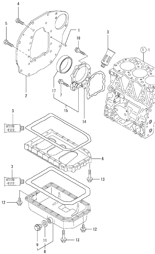
Fig.3. MOUNTING FLANGE & OIL SUMP
