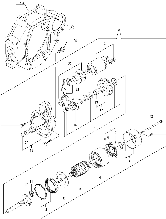
Fig.15. STARTER MOTOR
