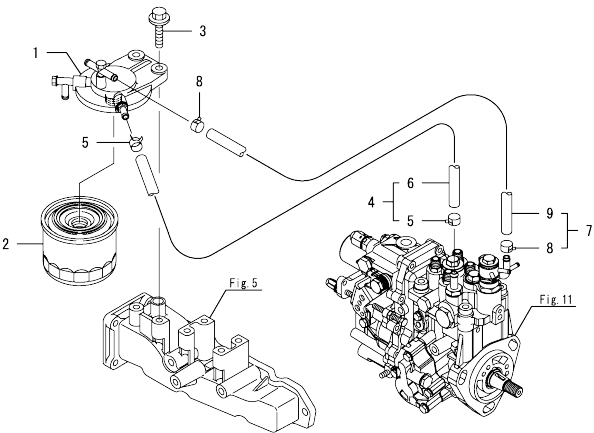
Fig.14. FUEL PIPE
