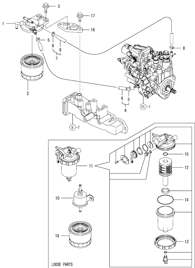
Fig.14. FUEL PIPING
