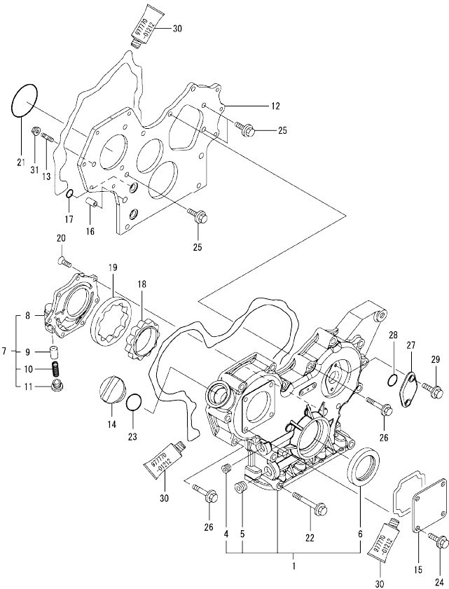
Fig.2. GEAR HOUSING
