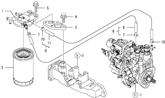
Fig.14. FUEL PIPING
