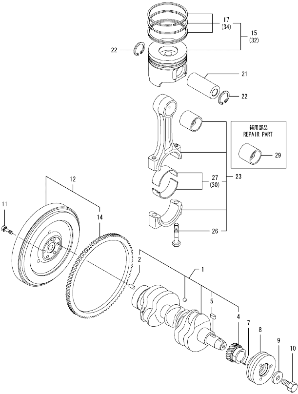
0CW10-M57800 ENGINE Fig.8. CRANKSHAFT & PISTON
