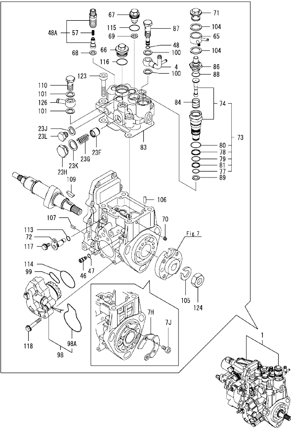
Fig.17. FUEL INJECTION PUMP(INNER PARTS)
