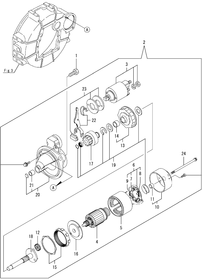
Fig.14. STARTER MOTOR
