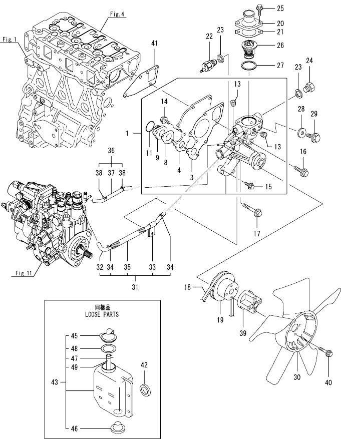
OCD10-M81202 3TNV82A-SYB/3TNV82A-SYBT Fig.10. COOLING WATER SYSTEM
