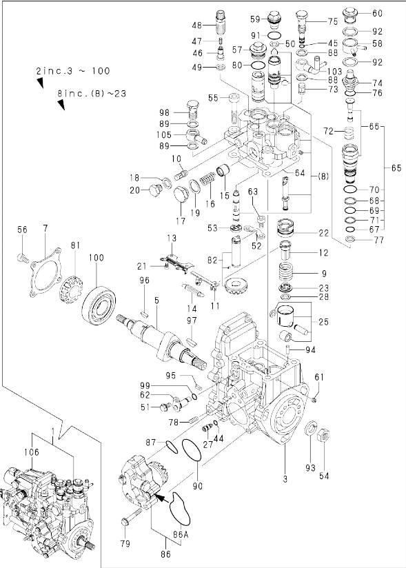
Fig.1. FUEL INJECTION PUMP
