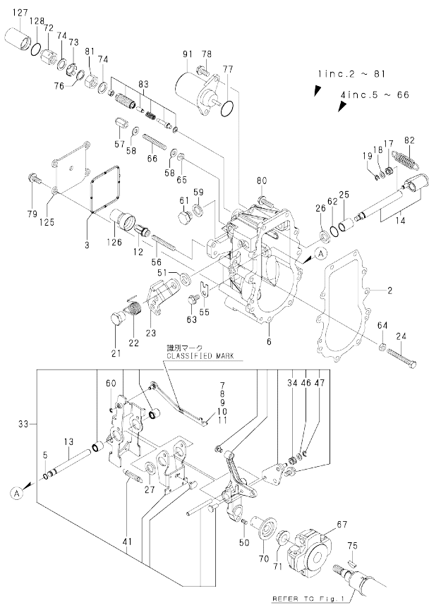
Fig.2. GOVERNOR
