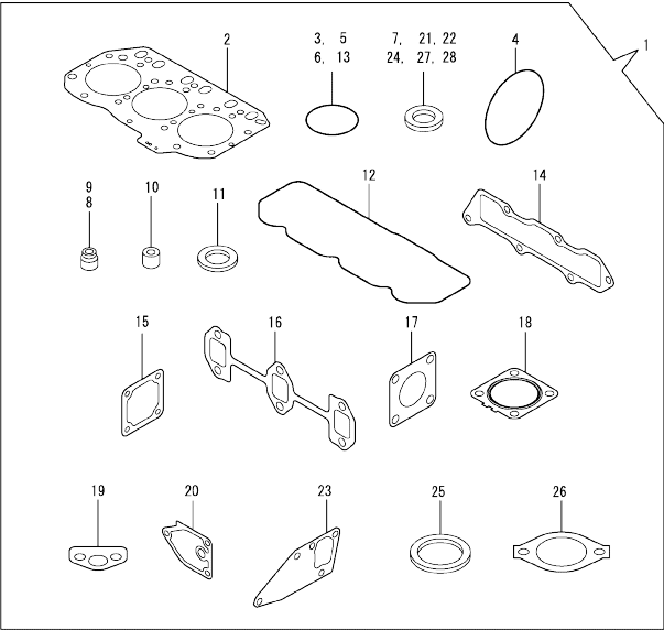
Fig.17. GASKET SET
