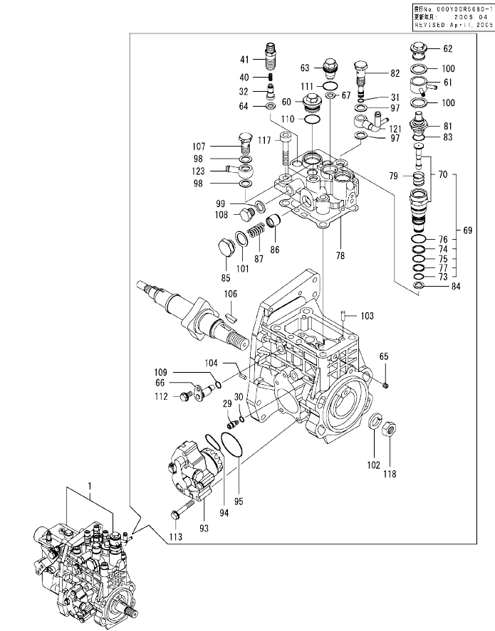
Fig.21. FUEL INJECTION PUMP(INNER PARTS)
