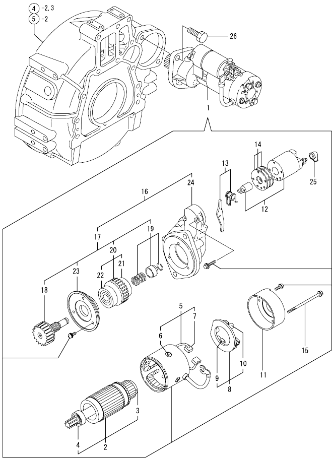
Fig.18. STARTER MOTOR
