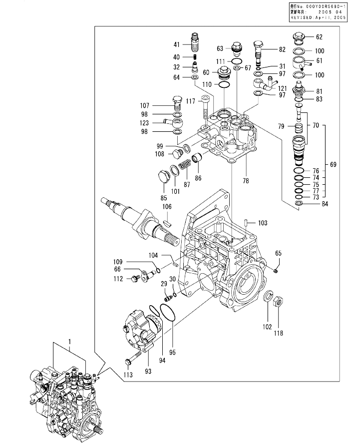
Fig.23. FUEL INJECTION PUMP(INNER PARTS)
