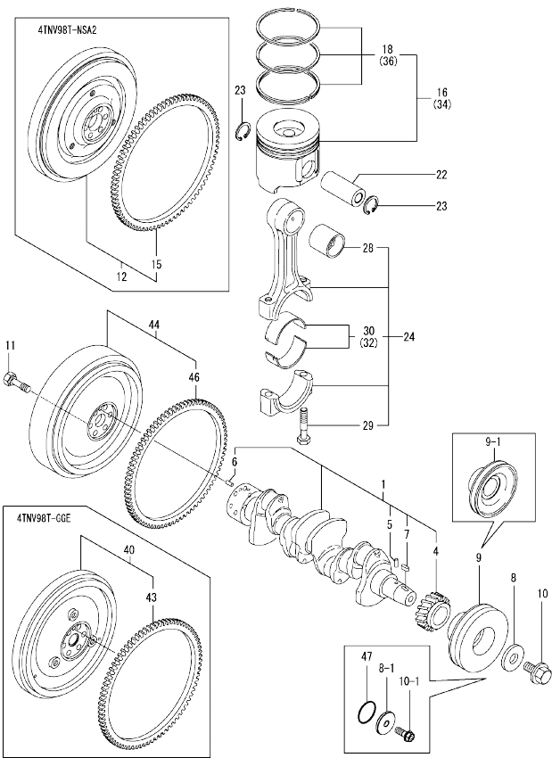
Fig.11. CRANKSHAFT & PISTON
