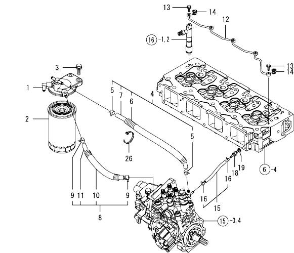
Fig.17. FUEL PIPING
