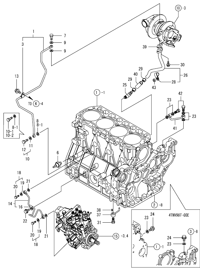
Fig.13. LUB. OIL PIPING
