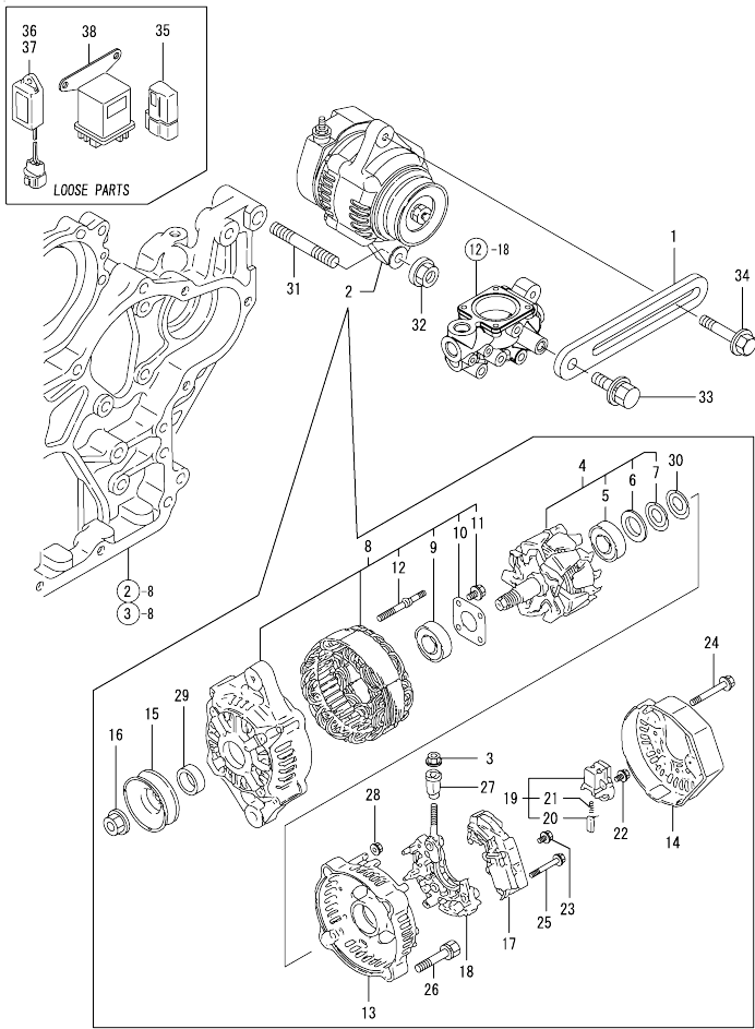
OCR10-M56800 ENGINE Fig.19. GENERATOR
