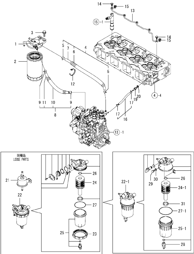
Fig.16. FUEL LINE
