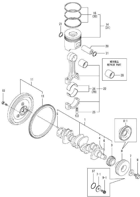
Fig.9. CRANKSHAFT & PISTON
