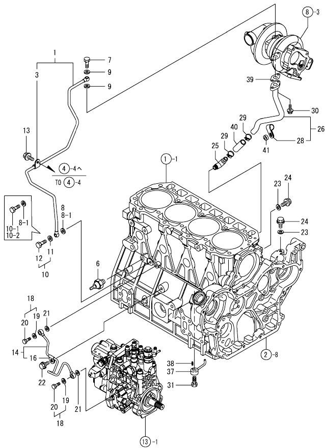
Fig.11. LUB.OIL LINE
