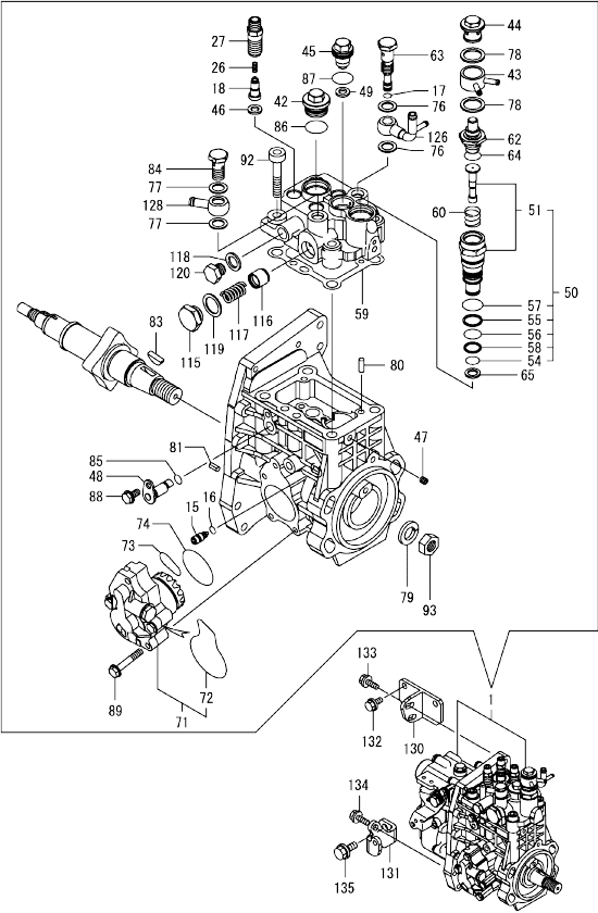
Fig.13. FUEL INJECTION PUMP
