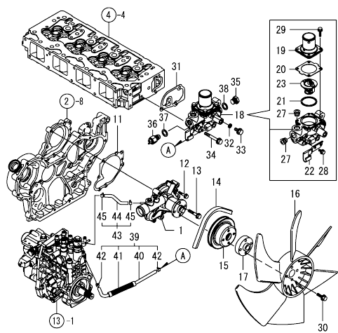
Fig.12. COOLING WATER SYSTEM
