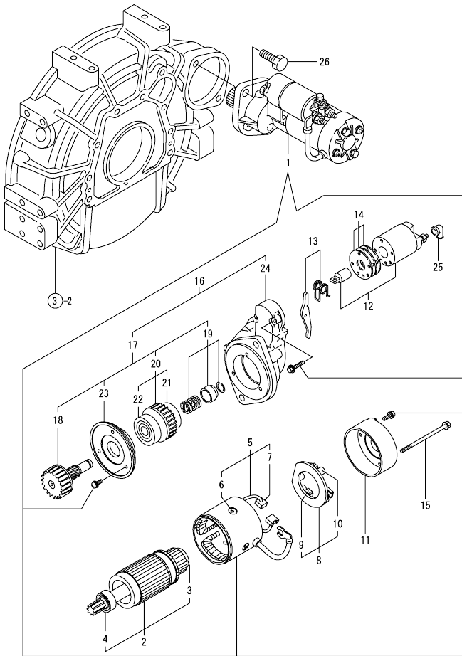
Fig.17. STARTING MOTOR
