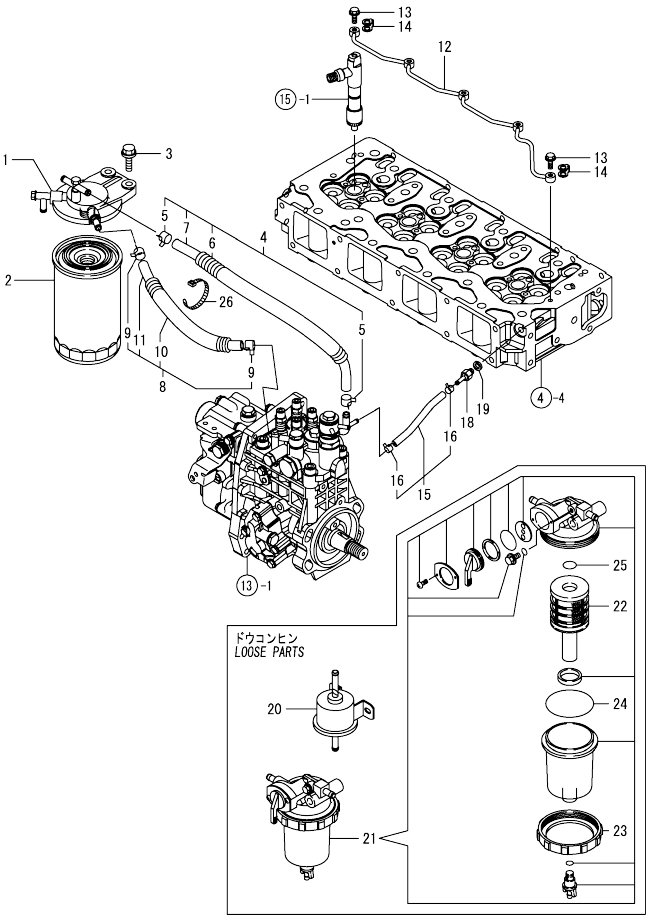
Fig.16. FUEL LINE
