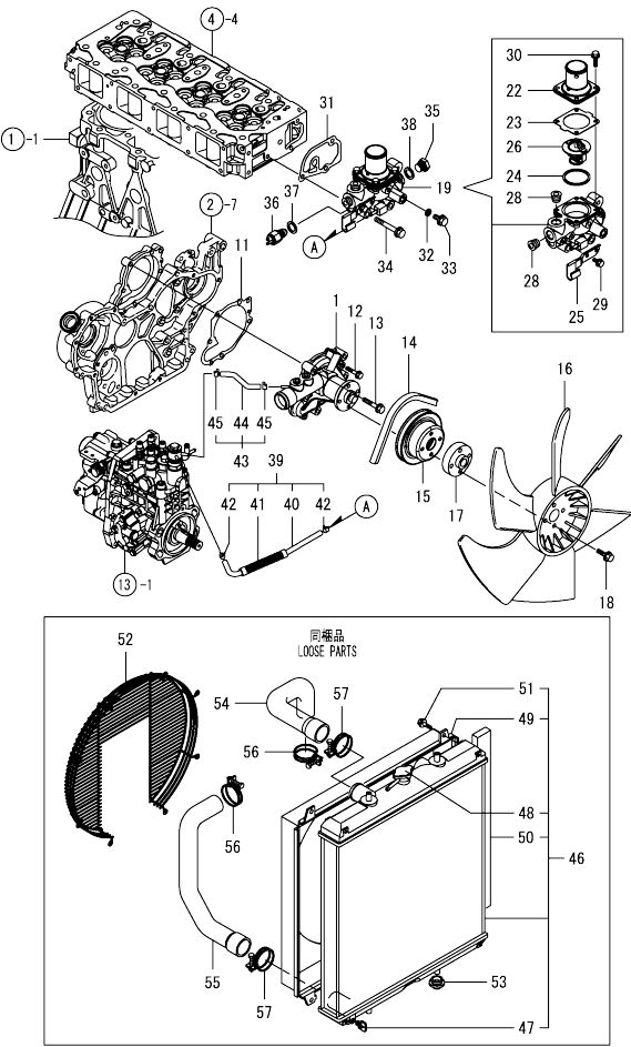
Fig.12. COOLING WATER SYSTEM
