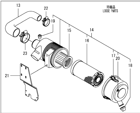
Fig.5. SUCTION MANIFOLD & AIR CLEANER
