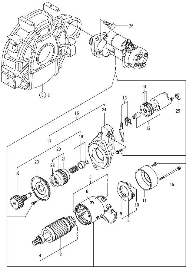
Fig.17. STARTING MOTOR
