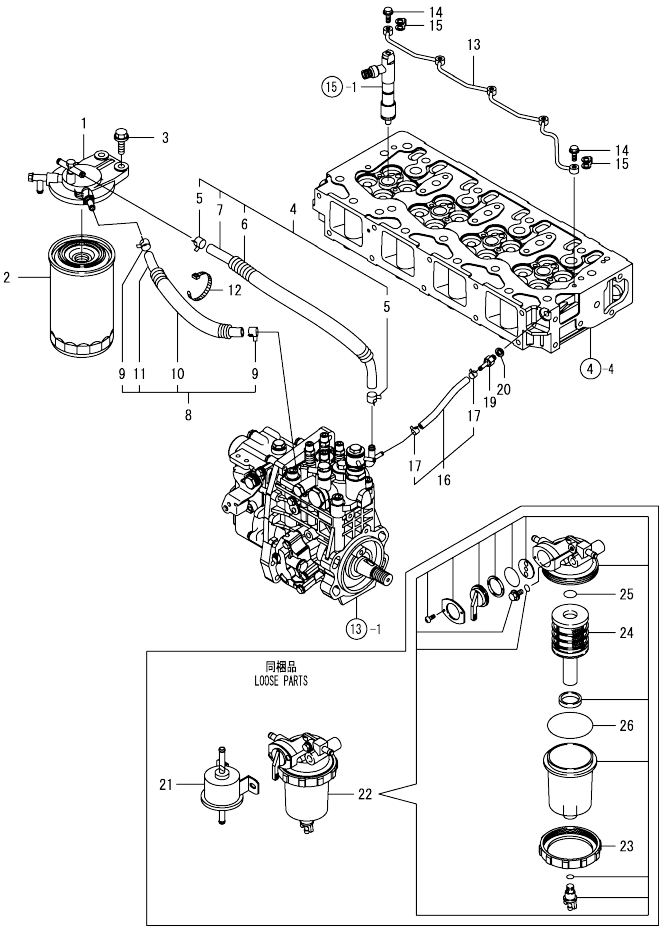
Fig.16. FUEL LINE
