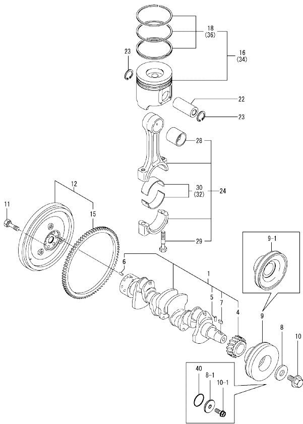
Fig.9. CRANKSHAFT & PISTON
