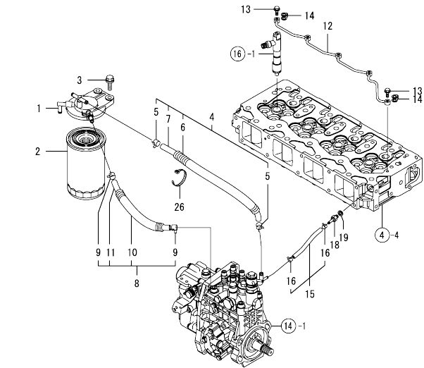
OCR10-M65300 ENGINE Fig.17. FUEL PIPE
