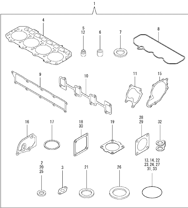
Fig.22. GASKET SET
