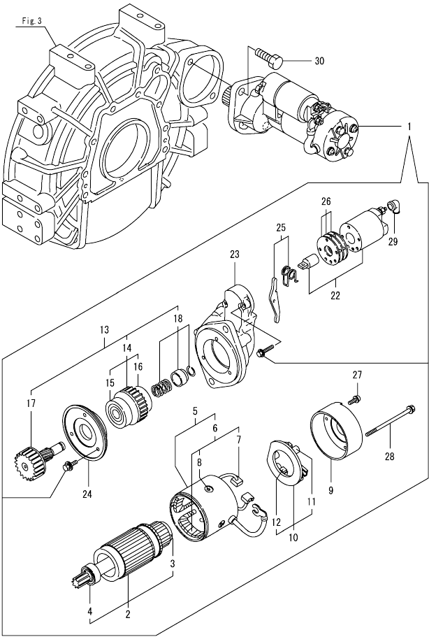
Fig.23. (19A)STARTER MOTOR
