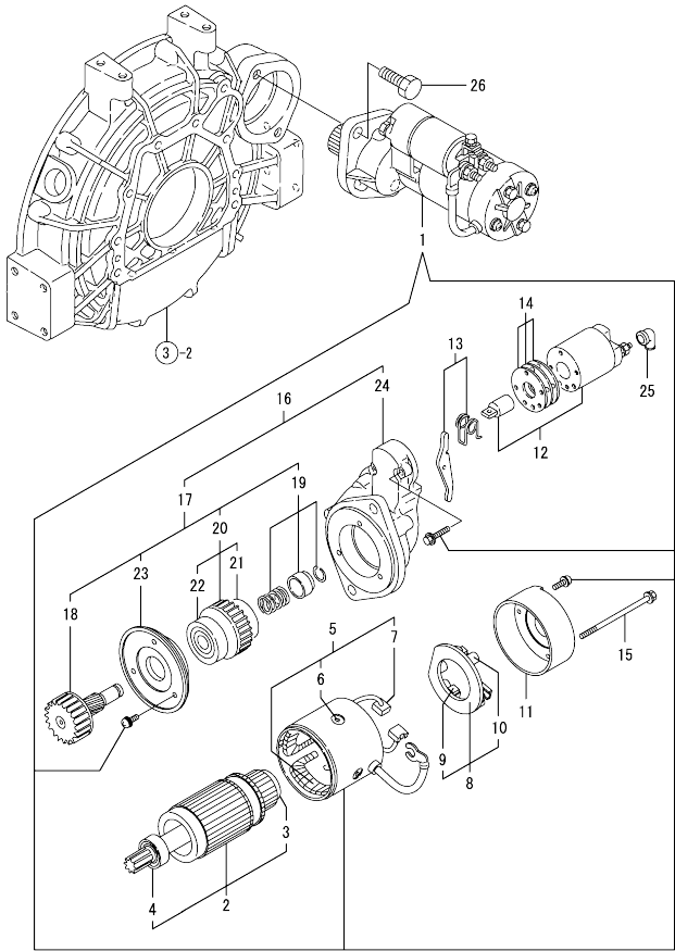
0CW10-M14800 4TNV98T-GKL Fig.17. STARTING MOTOR
