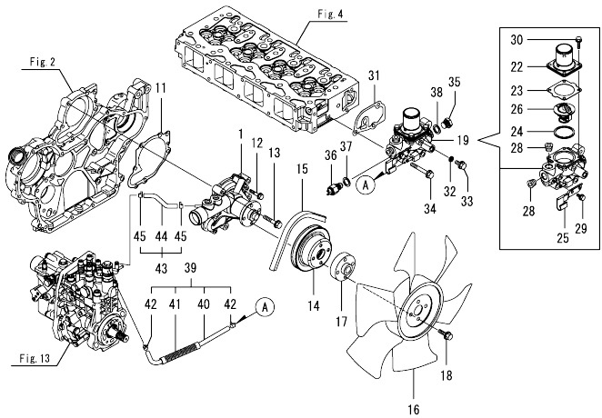
Fig.12. COOLING WATER SYSTEM
