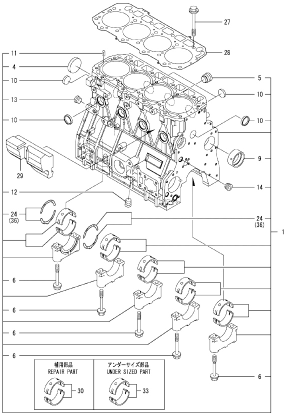
0CW10-M67300 4TNV98T-GPGEC Fig.1. CYLINDER BLOCK
