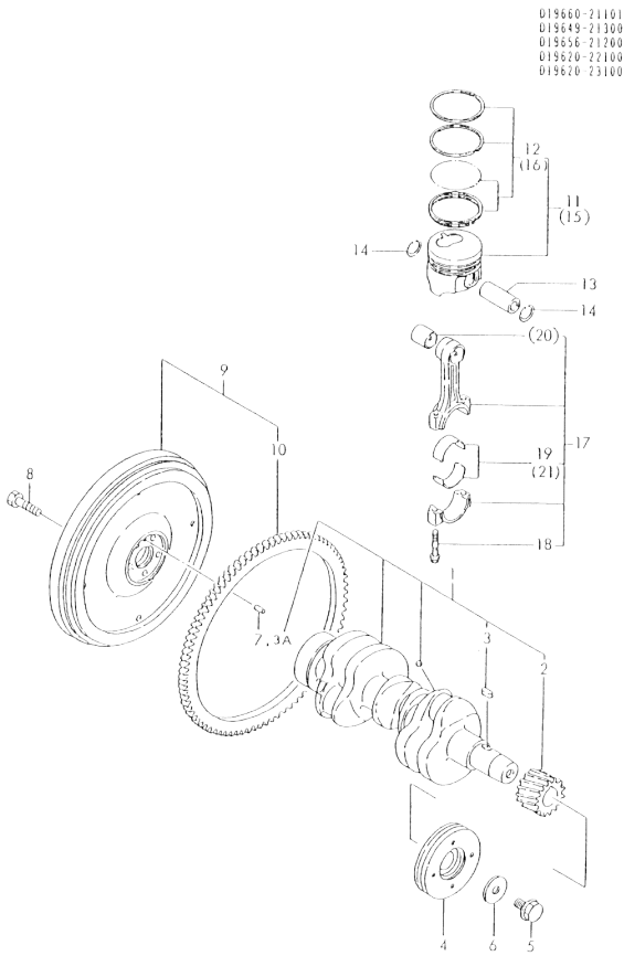
Fig.53. CRANKSHAFT & PISTON
