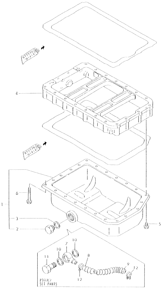
Fig.5. LUB.OIL SUMP
