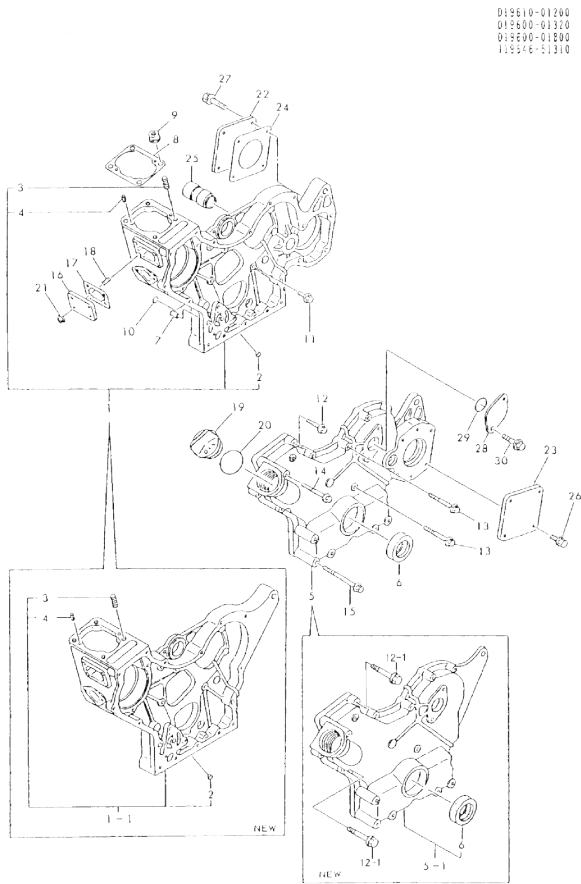
Fig.47. GEAR HOUSING
