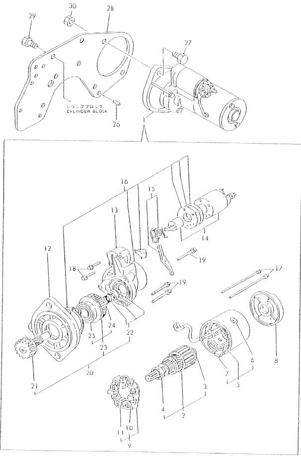
Fig.59. STARTING MOTOR
