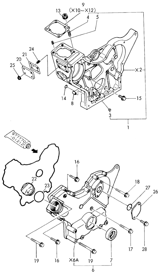
Fig.2 GEAR HOUSING
