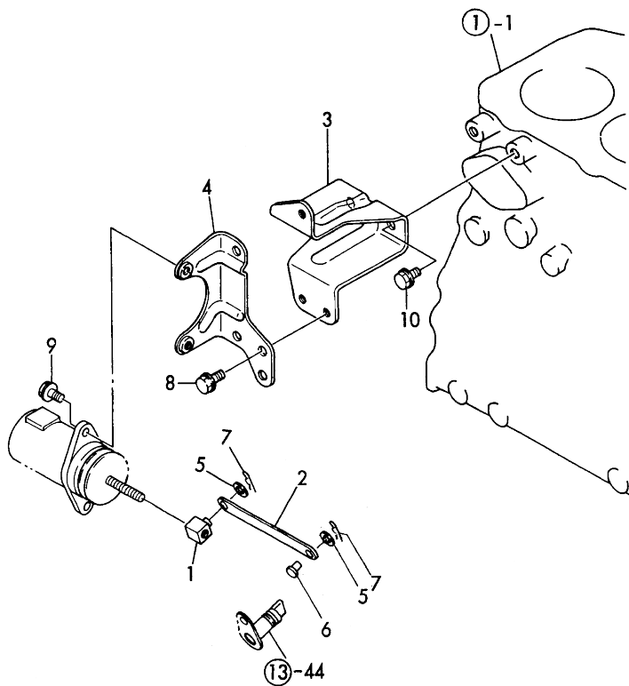
Fig. 13 ENGINE STOP DEVICE
