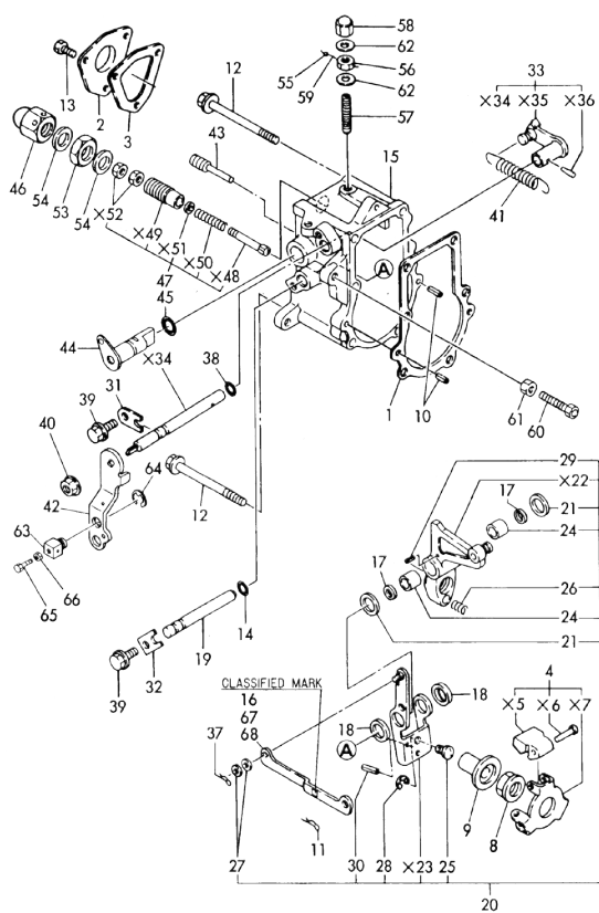
Fig. 12 GOVERNOR
