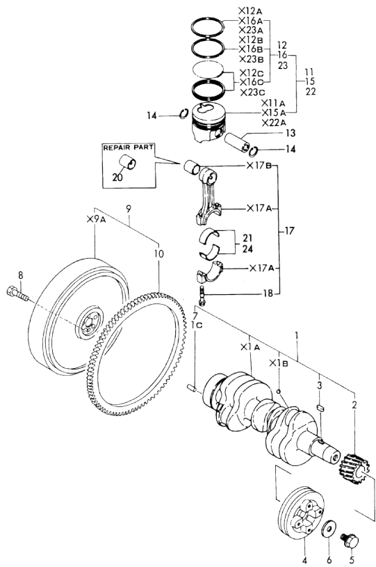
Fig.7 CRANKSHAFT & PISTON
