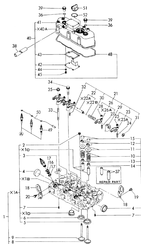
Fig. 4 CYLINDER HEAD & BONNET
