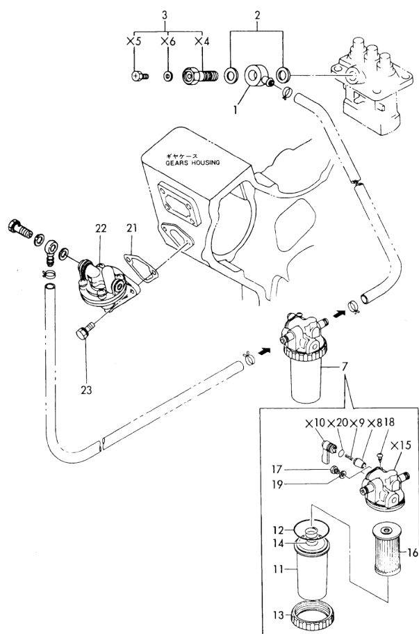
Fig. 11 FUEL LINE
