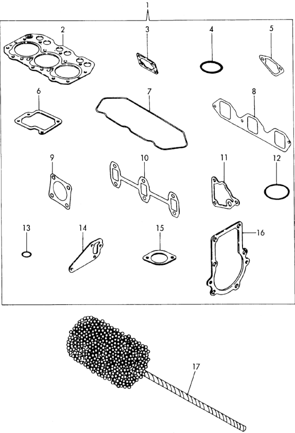
Fig.16 GASKET SET & TOOL (OPTIONAL)
