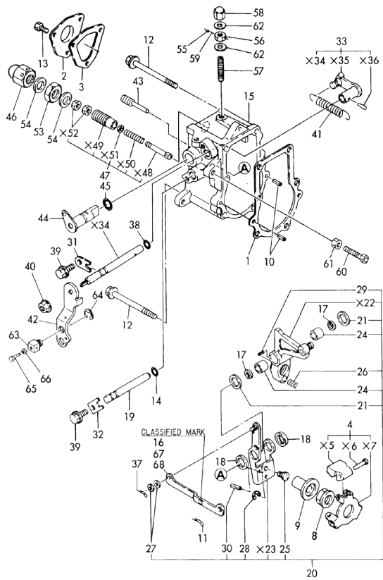
Fig.12 GOVERNOR
