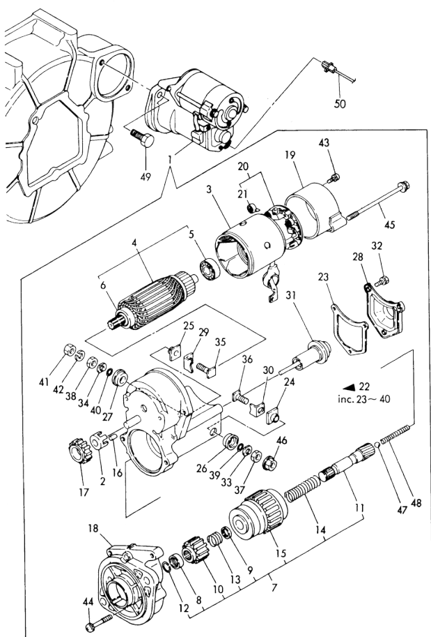
Fig. 14 STARTING MOTOR
