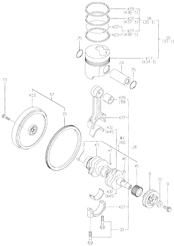
Fig.9. CRANKSHAFT & PISTON
