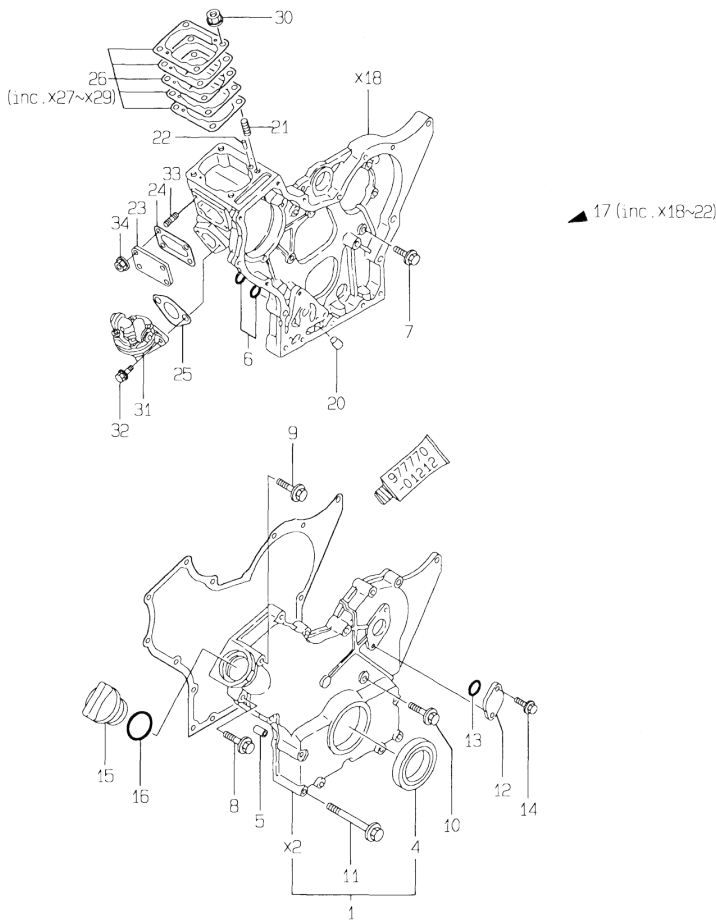
Fig.2. GEAR HOUSING
