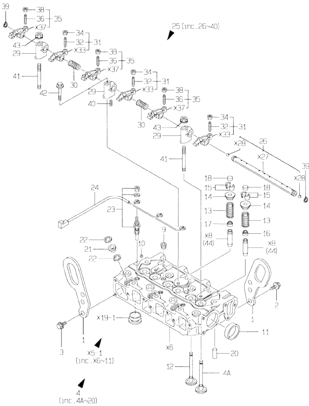
Fig.5. CYLINDER HEAD
