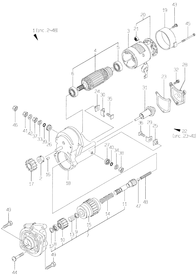
Fig.16. STARTING MOTOR
